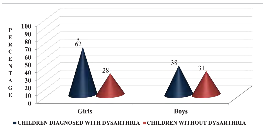
Fig. 1. DUFS (fatigue assessment scale).
